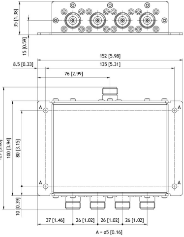
MOUNTING DETAILS (Dimensions excl. cover)
